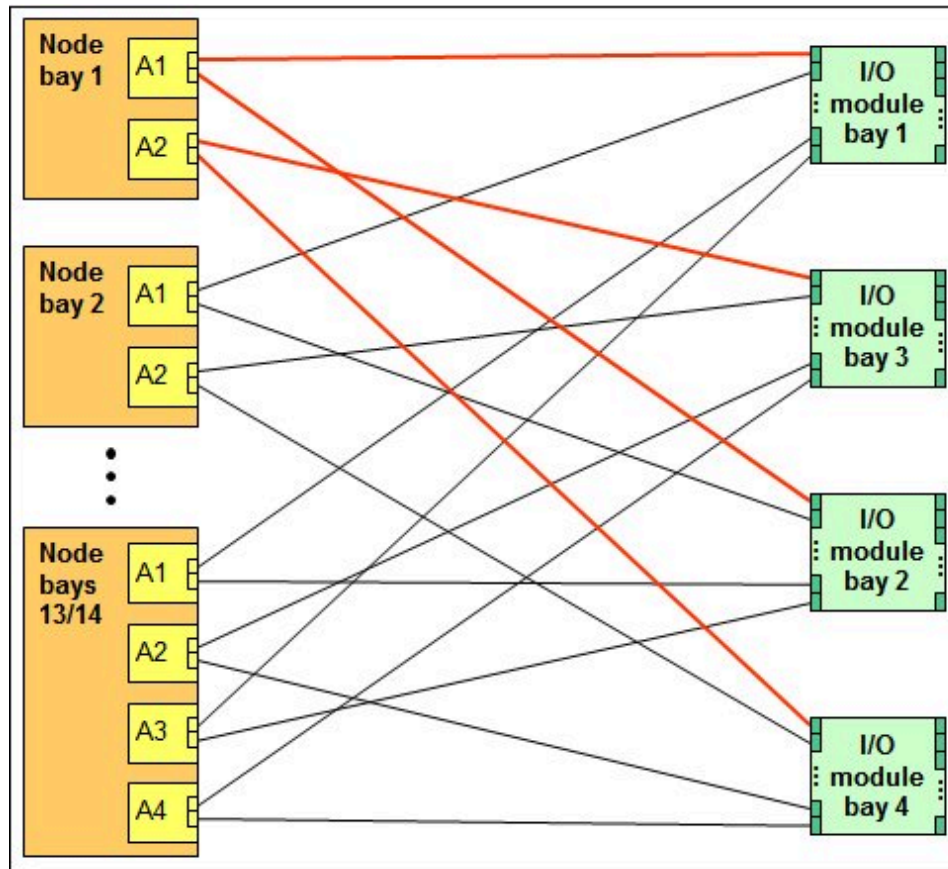
Figure 3. Logical layout
